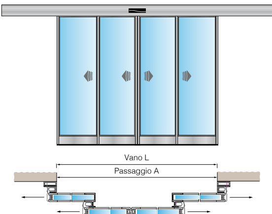
TSA BILATERAL 4 ANTE MOBILI
